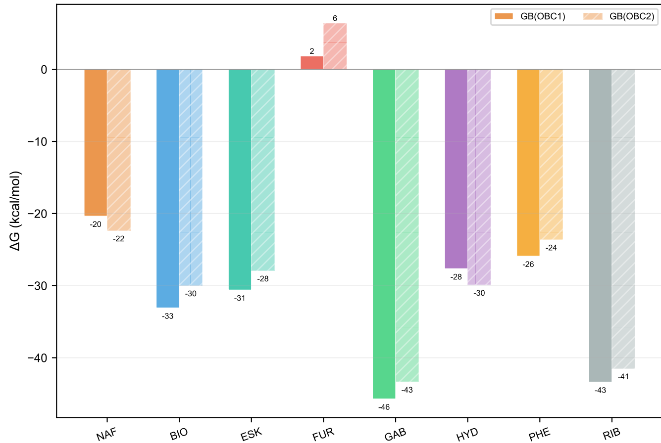
a. Absolute binding free energies
