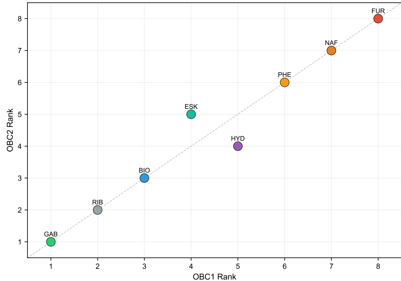
b. Rank correlation (Spearman \rho=0.976 , p=3.31e-05 )
